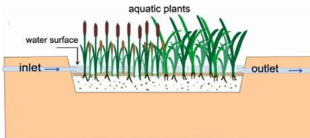
Fig. 3. Schematic of a free-surface flow CW
