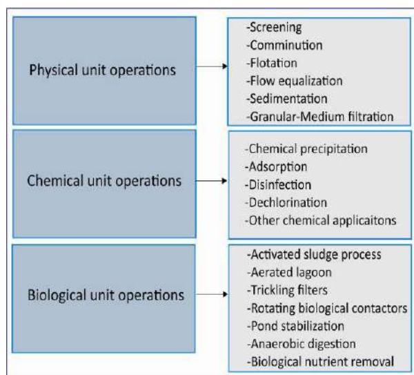
Fig. 1. Wastewater treatment unit operations and processes
