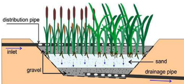
Fig. 4. Schematic of a vertical flow CW
