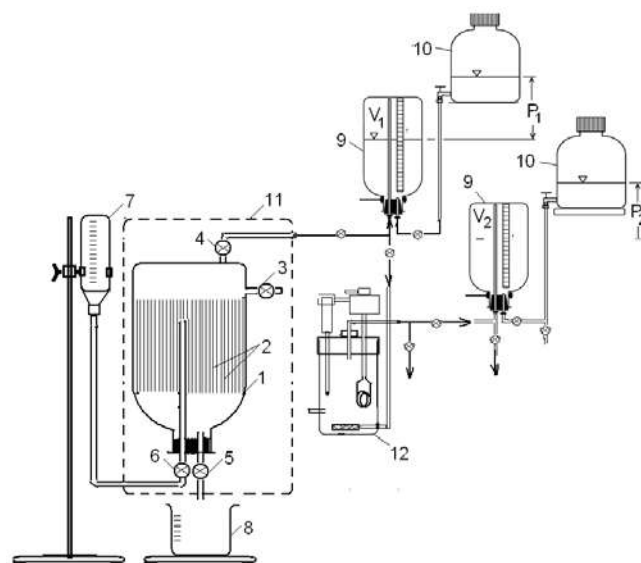
Fig. 1. The scheme of bench-scale reactor for biochemical generation of biogas and its purification from the admixtures: 1 – bioreactor; 2 – package for the immobilization of microorganisms; 3 – 6 – valves; 7 – reservoir for nutrient solution; 8 – glass; 9 – reservoir with calibrated capacity; 10 – water reservoirs; 11 – thermostat; 12 – device for biogas purification.
