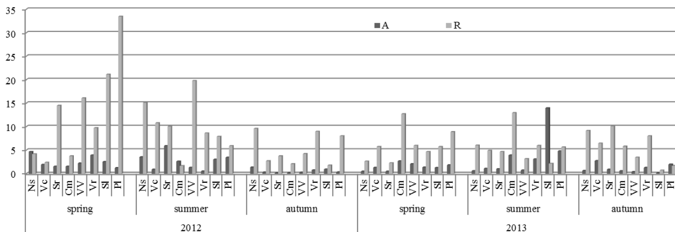
Figure 2. Seasonal dynamics of the phytoplankton primary production (A – gO 2 /m 2 ·24 h) and organic matter destruction (R – gO 2 /m 2 ·24 h) values in the Dniester River (Ns-Naslavcea, Vc – Volcinet, Sr – Soroca, Cm – Camenca, VV – Vadul-lui-Voda, Vr – Varnita, SI – Sucleia, PI – Palanca) in 2012-2013 years
